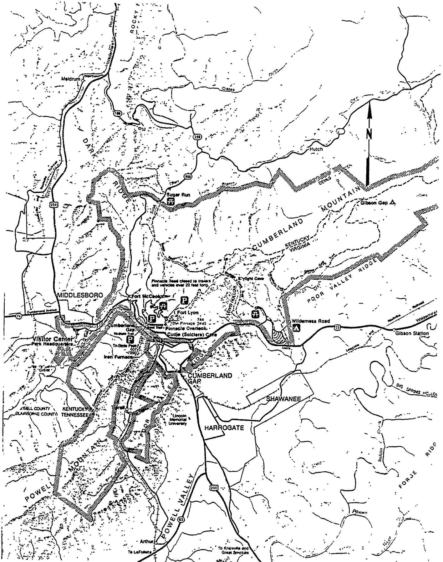
Figure 4.5 Map of Cumberland Gap (NPS).
