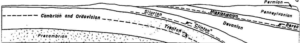
GEOLOGIC MAP AND CROSS SECTION OF OHIO
