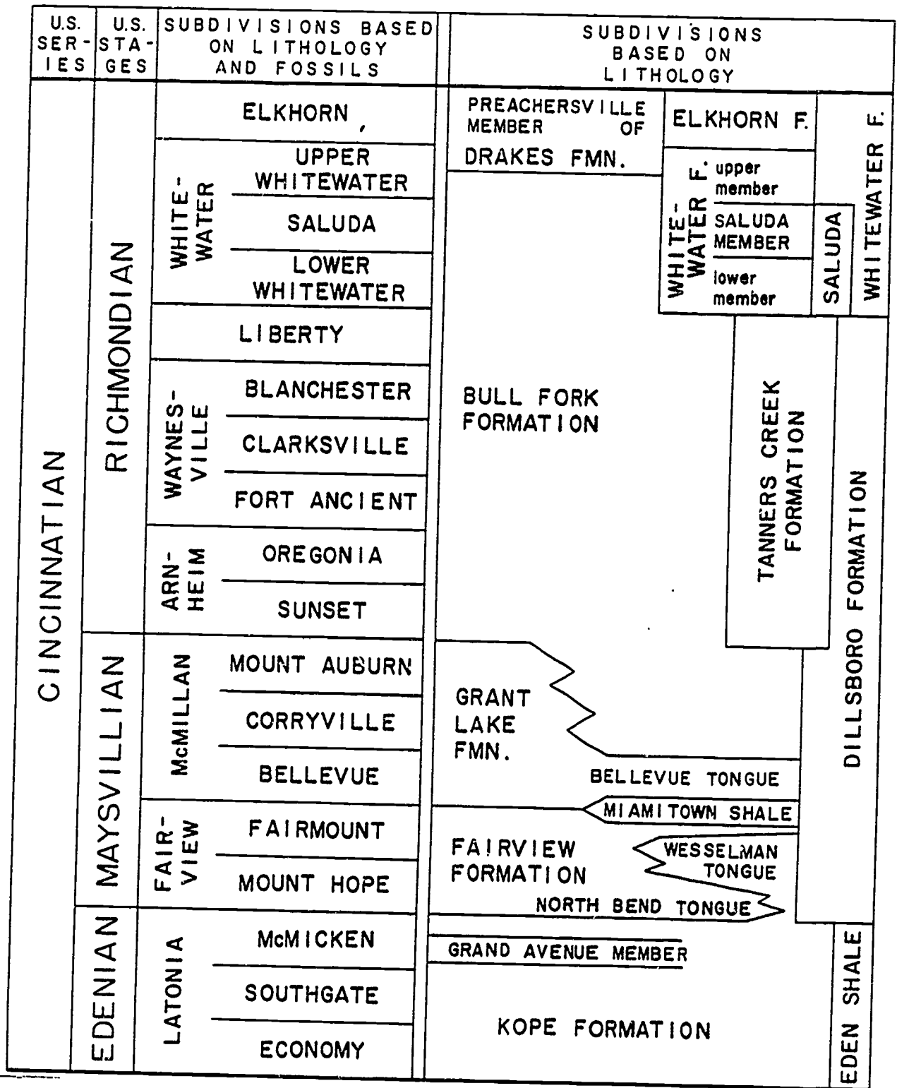
Figure 5.5 Stratigraphy in the Maysville area. The relationship of stratigraphic names that have been applied to rocks in the Indiana, Kentucky and Ohio area is shown on the right side of the diagram. These names do not necessarily represent different rock units or their lateral relationships. Data derived from: Caster, Dalve, and Pope (1955/61) and Anstey and Fowler (1969), Brown and Lineback (1966), Ford (1967,1974), Gray (1972), Hatfield (1968), Hay et al. (1981), Martin (1975), Peck (1966), and Ross et al. (1982). (Reprinted from Davis, 1981, with permission.)
