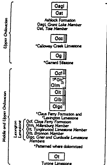
Figure 5.4 Kentucky River Fault System (Boonesborough Fault portion) (Black, MacQuown and DeHaas, 1981).
