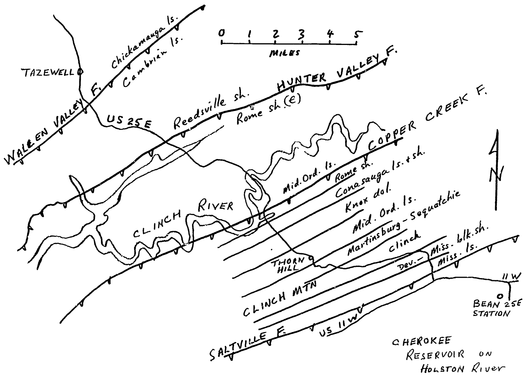
Figure 4.2 Thrust faults in the Valley and Ridge between Cherokee Reservoir and Tazewell .
