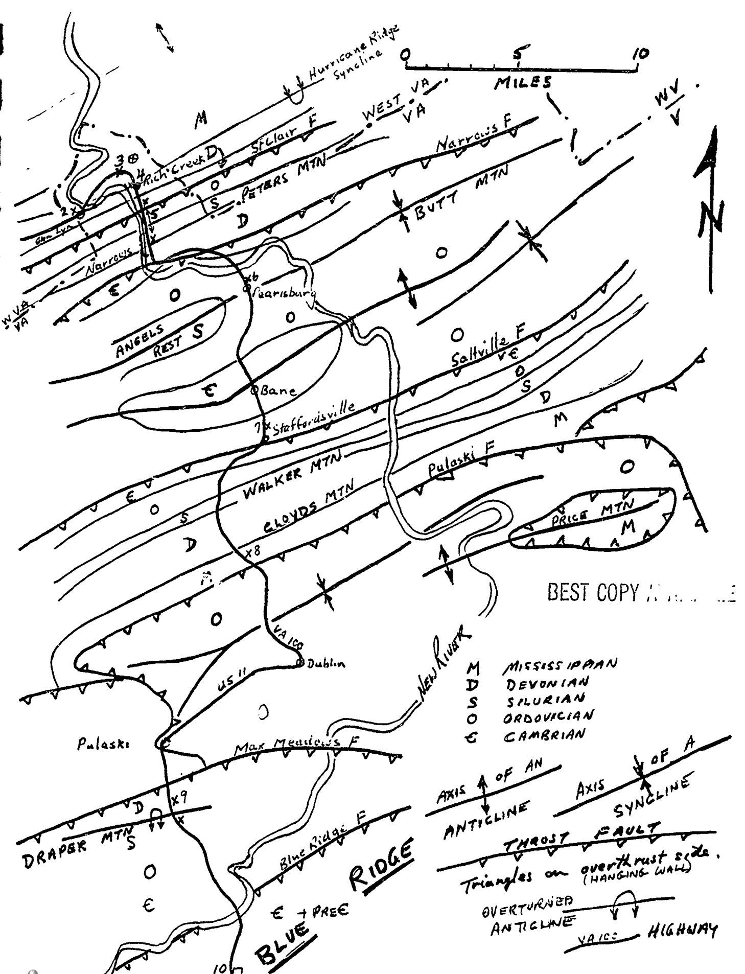
Figure 2.2 Geologic sketch map of Valley and Ridge Province from Glen Lyn to Sylvatus.
