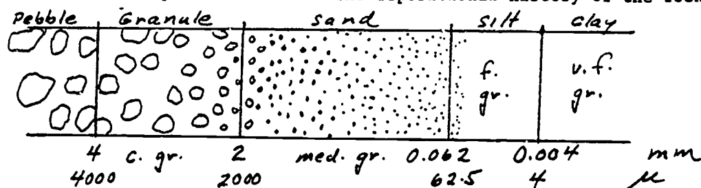
Figure 7. Particle sizes for classification of sedimentary rocks.
