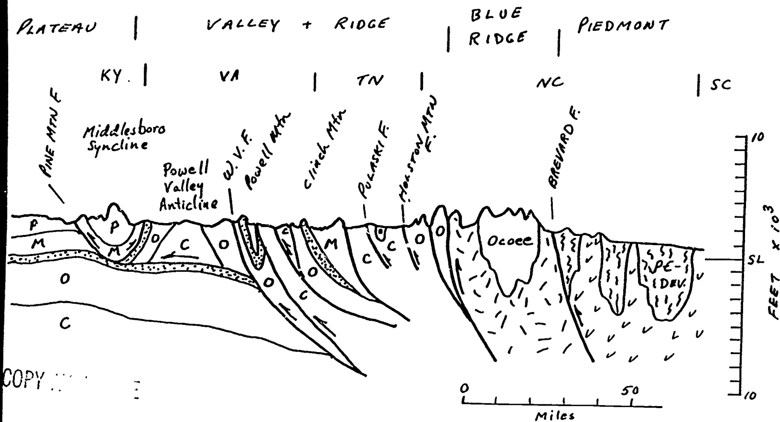
Figure 4.4 Powell Valley anticline and Appalachian cross section from Plateau to Piedmont (KY - SC). NW -SE section through Kingsport, TN. State Boundaries approximate. Vertical exaggeration: 20X. (Modified from Renfro and Feray, 1970).
