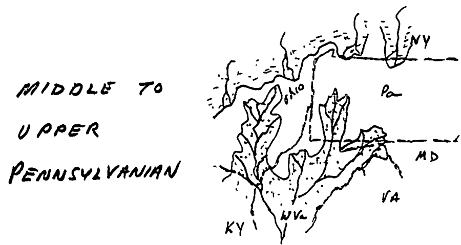
Figure 1.4 Paleogeography of the Appalachian Basin during the Pennsylvanian (modified from Donaldson, 1972).
