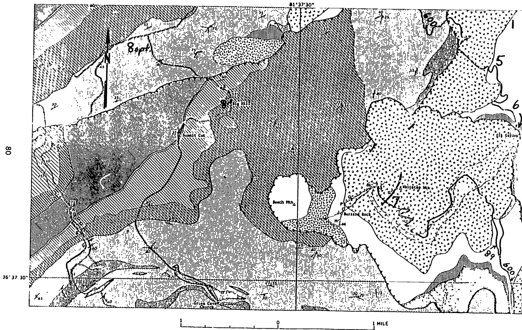
Figure 3.61 Geology of Whitetop Mountain area (Rankin, 1967).
