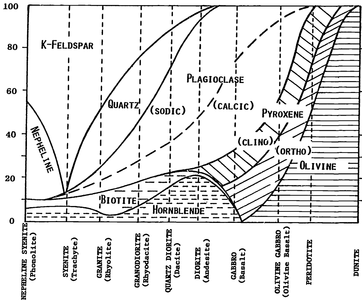
APPENDIX A CLASSIFICATION OF IGNEOUS ROCKS. Extrusive equivalents in parentheses.
