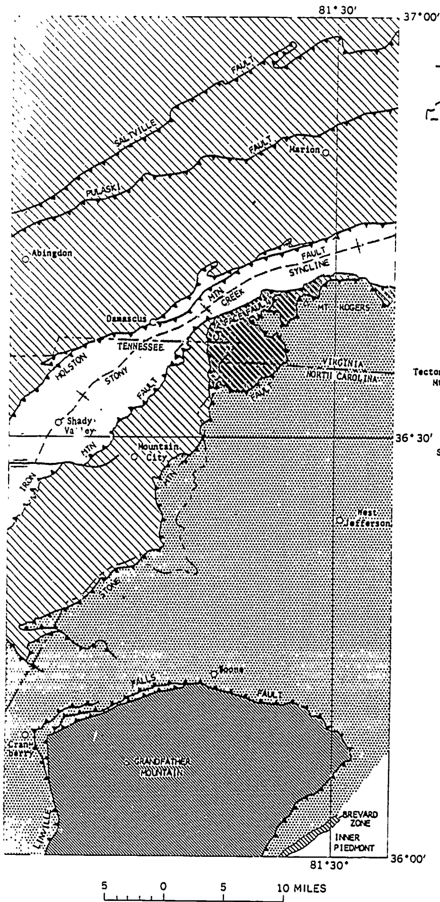
Figure 3.5 Geology of the Mt. Rogers area (Rankin, 1967).
