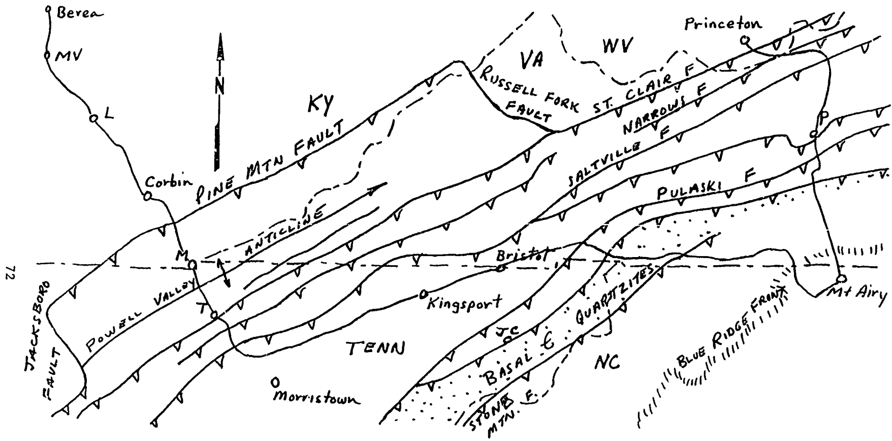
Figure 3.1 Major faults in the Valley and Ridge; itinerary for the second, third and fourth days.
