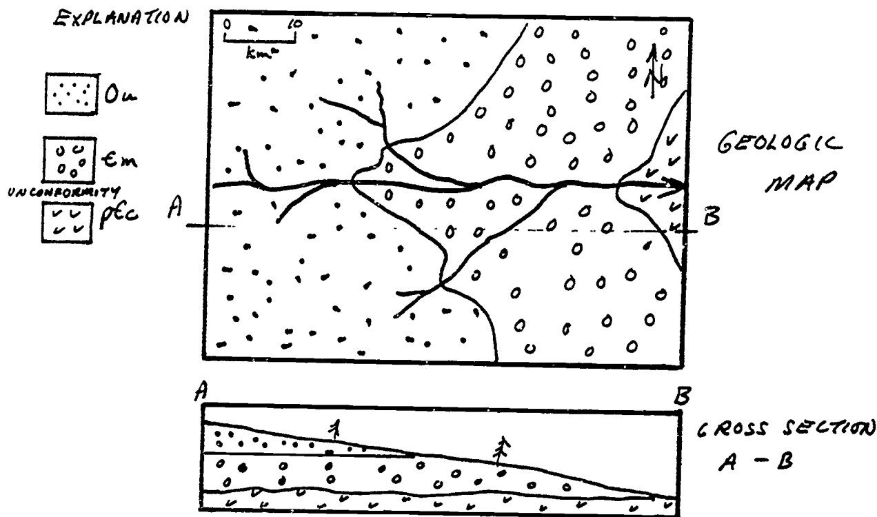
Figure 12. Geologic map and section -- horizontal strata. In the explanation, pcc = Precambrian crystallines, Em = Cambrian McKenzie Formation, and Ou = Ordovician Utgard Formation.
