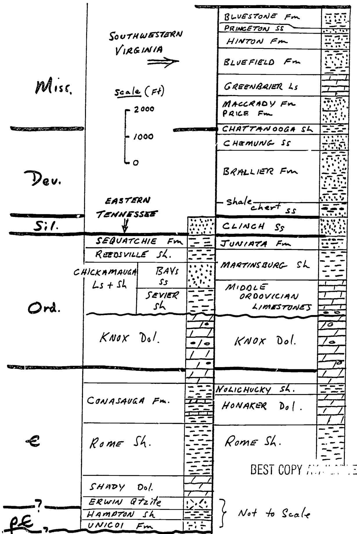
Figure 2.1 Geologic columns for Eastern Tennessee and Southwestern Virginia.
