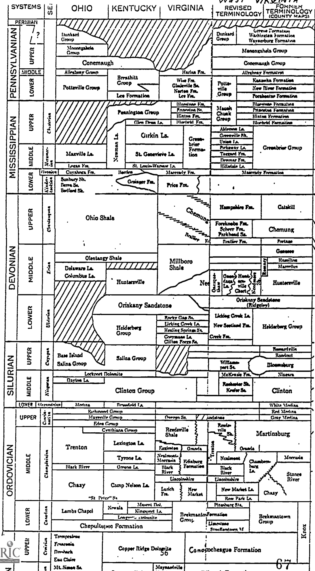
Figure 1.7. Correlation chart for Ohio, Kentucky, West Virginia and Virginia. (From WV Geol Survey, 1968).
