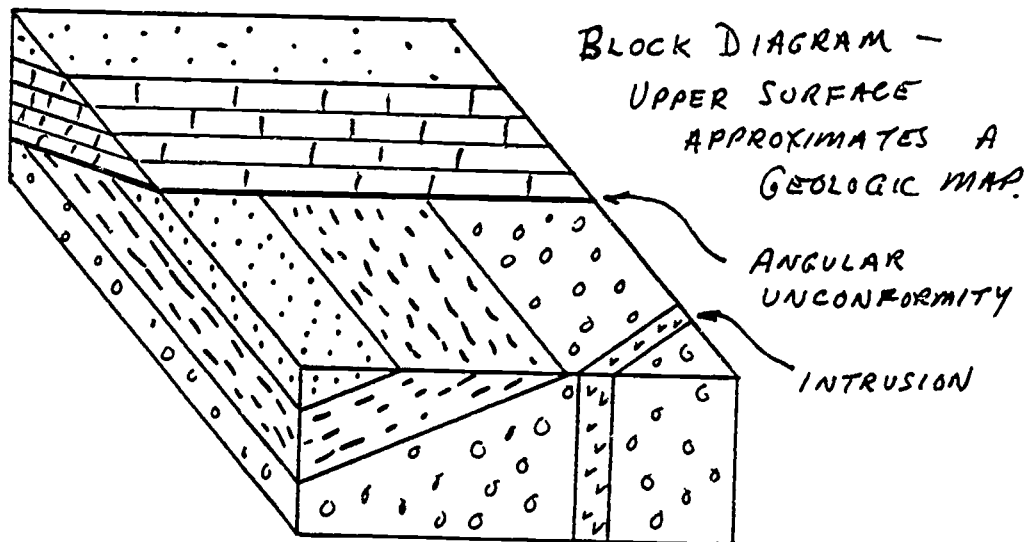
Figure 13. Block diagram showing inclined strata, angular unconformity and intrusion. (modified from Thomas, 1977).
