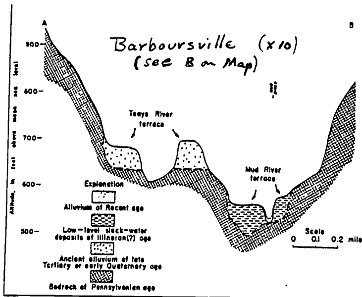
Figure 1.2 Teays River system (Modified from Rhodehamel and Carlston(1963).
